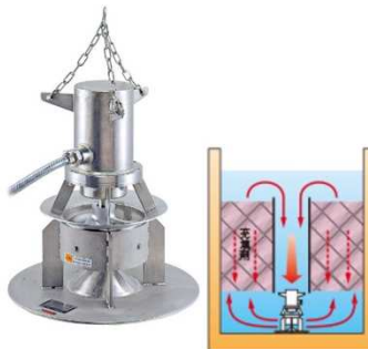
Downward stirrer
