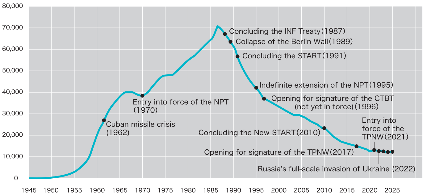
World Nuclear Arsenals:1945-2025 (estimated)
